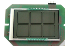
R10135-SC DISPLAY PANEL CONTROL VAC DIGITAL DISPLAY FOR VAC CONTROL PANEL
