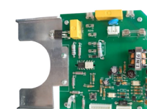
R10132-SC TARJETA ELECTRONICA VAC DIGITAL 1.6/1.8 PC BOARD VAC 1.6/1.8 DIGITAL
