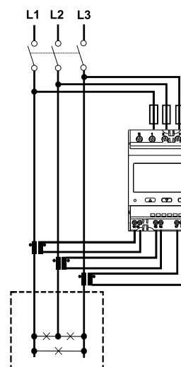
Fig. 10 Three-phase without neutral (3-wire).
